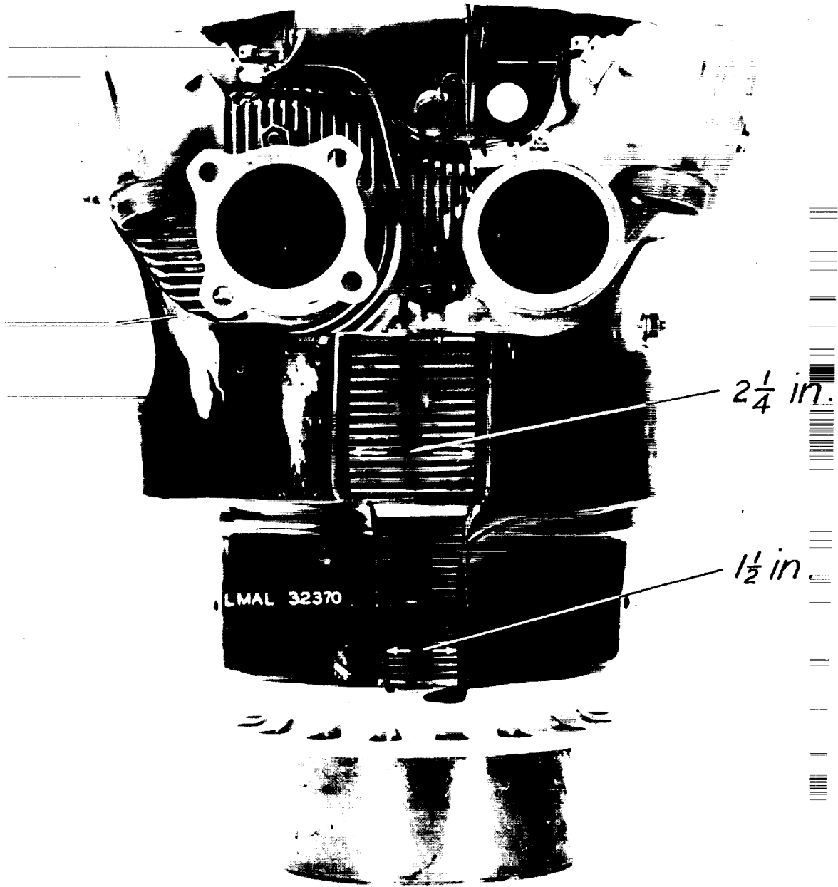
(b) Revised baffle. Arrow points to restriction at baffle outlet.
