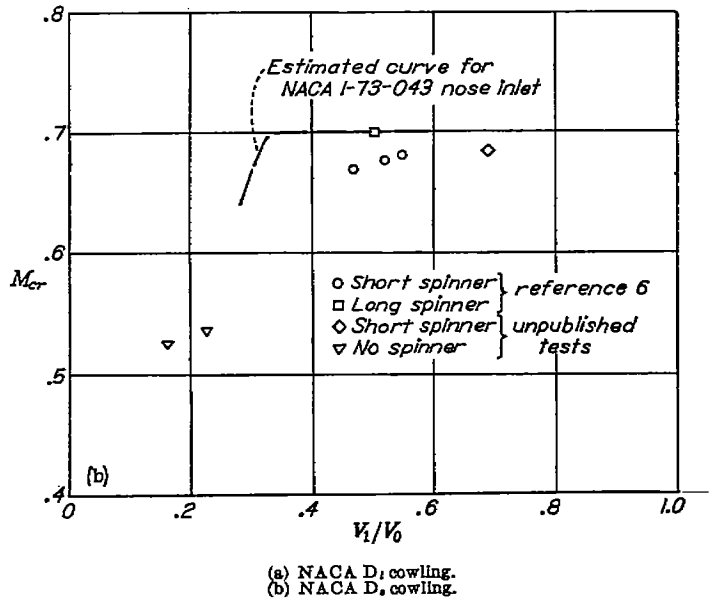
FIGURE 39.—Critical Mach numbers for NACA D 1 and D 2 cowlings. Estimated curves for NACA 1-series cowlings shown in figure 37 included for comparison. \alpha=0^\circ .
