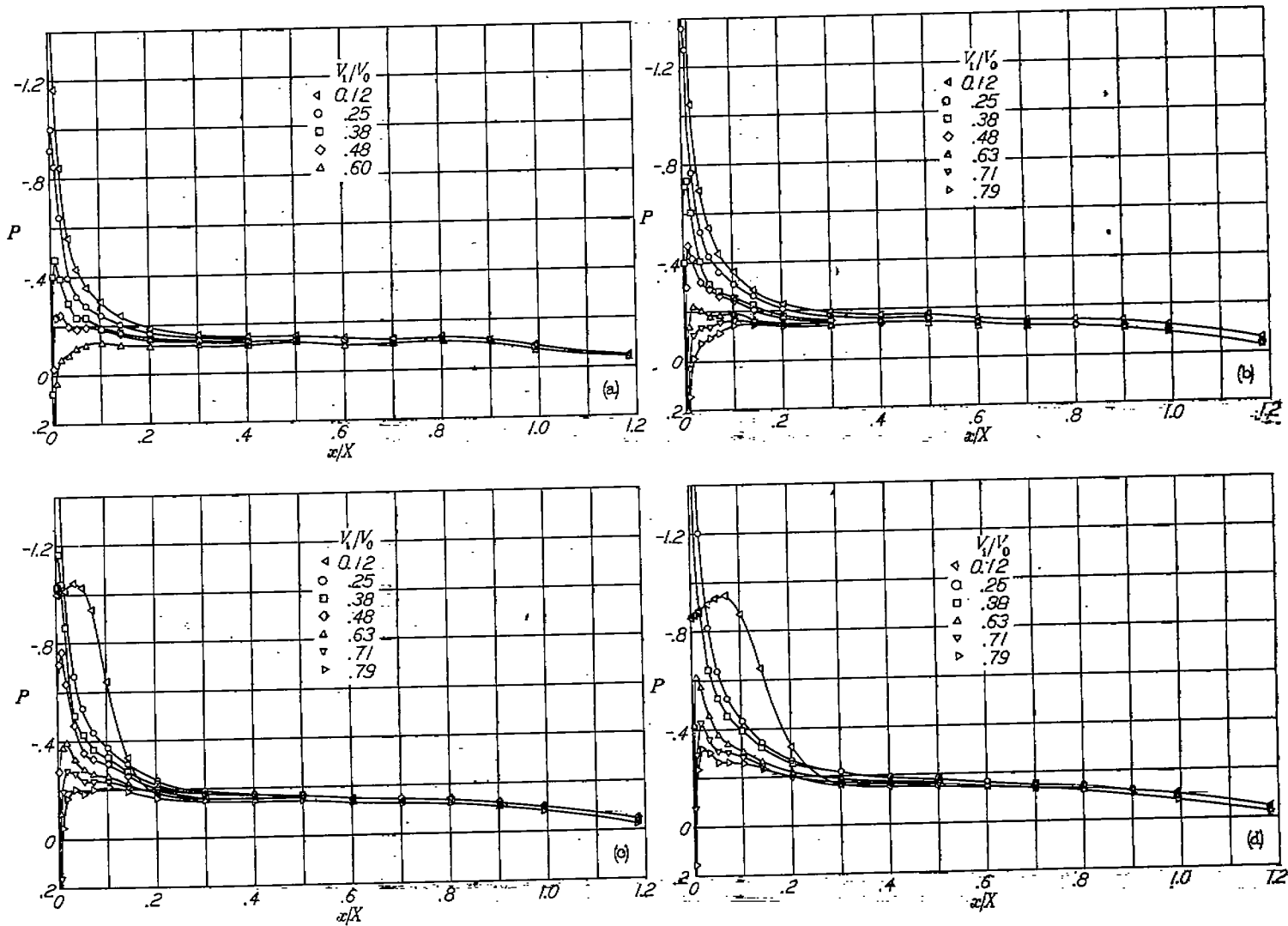
(a) \alpha = -0.1^\circ . (b) \alpha = 1.8^\circ . (c) \alpha = 3.9^\circ . (d) \alpha = 5.9^\circ . FIGURE 18.—Pressure distributions over the NACA 1-60-160 nose inlet. M_1 = 0.30 .
