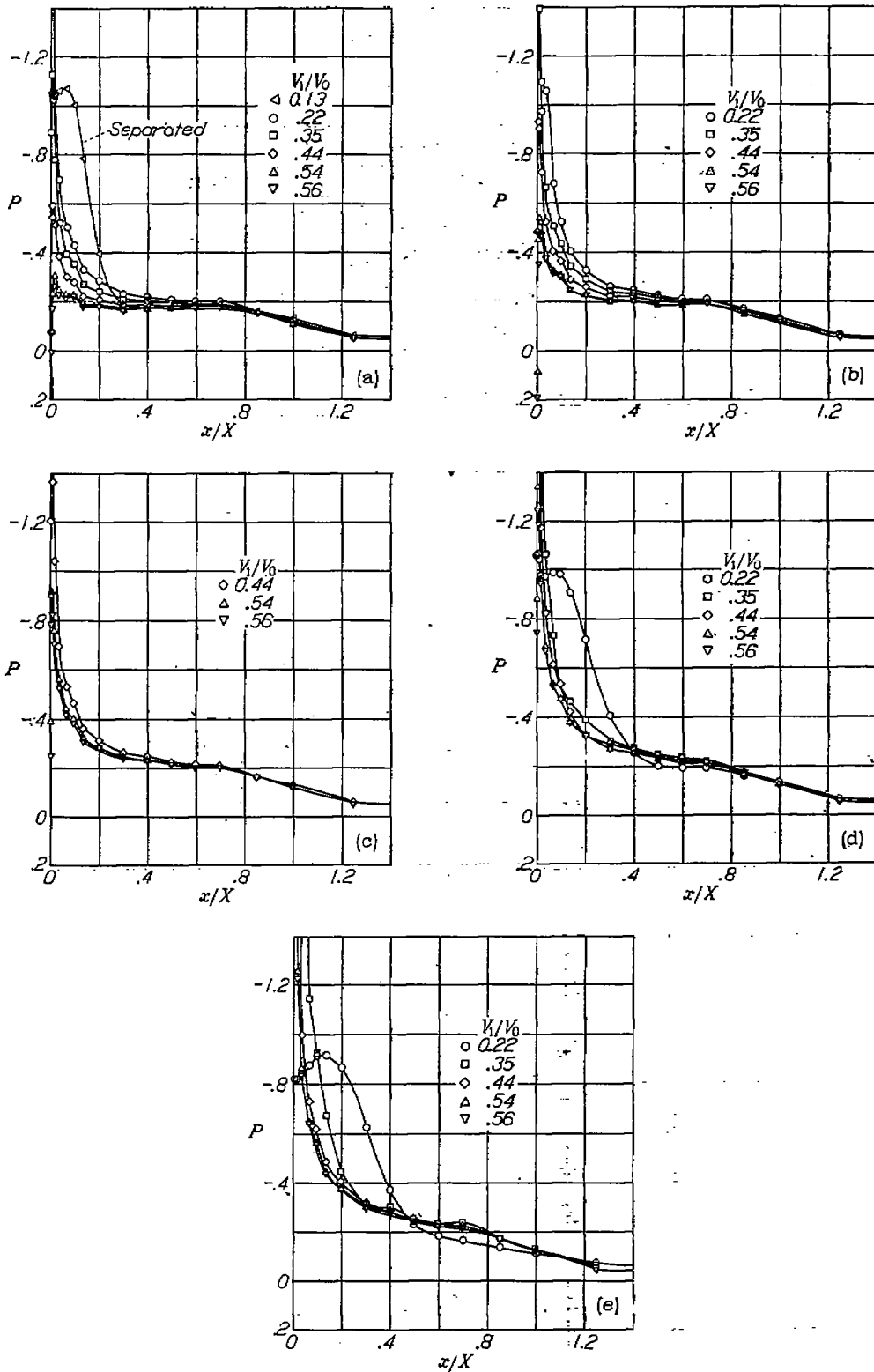
FIGURE 24.—Pressure distributions over the NACA 1-70-100 nose inlet. M_\infty = 0.40 .
