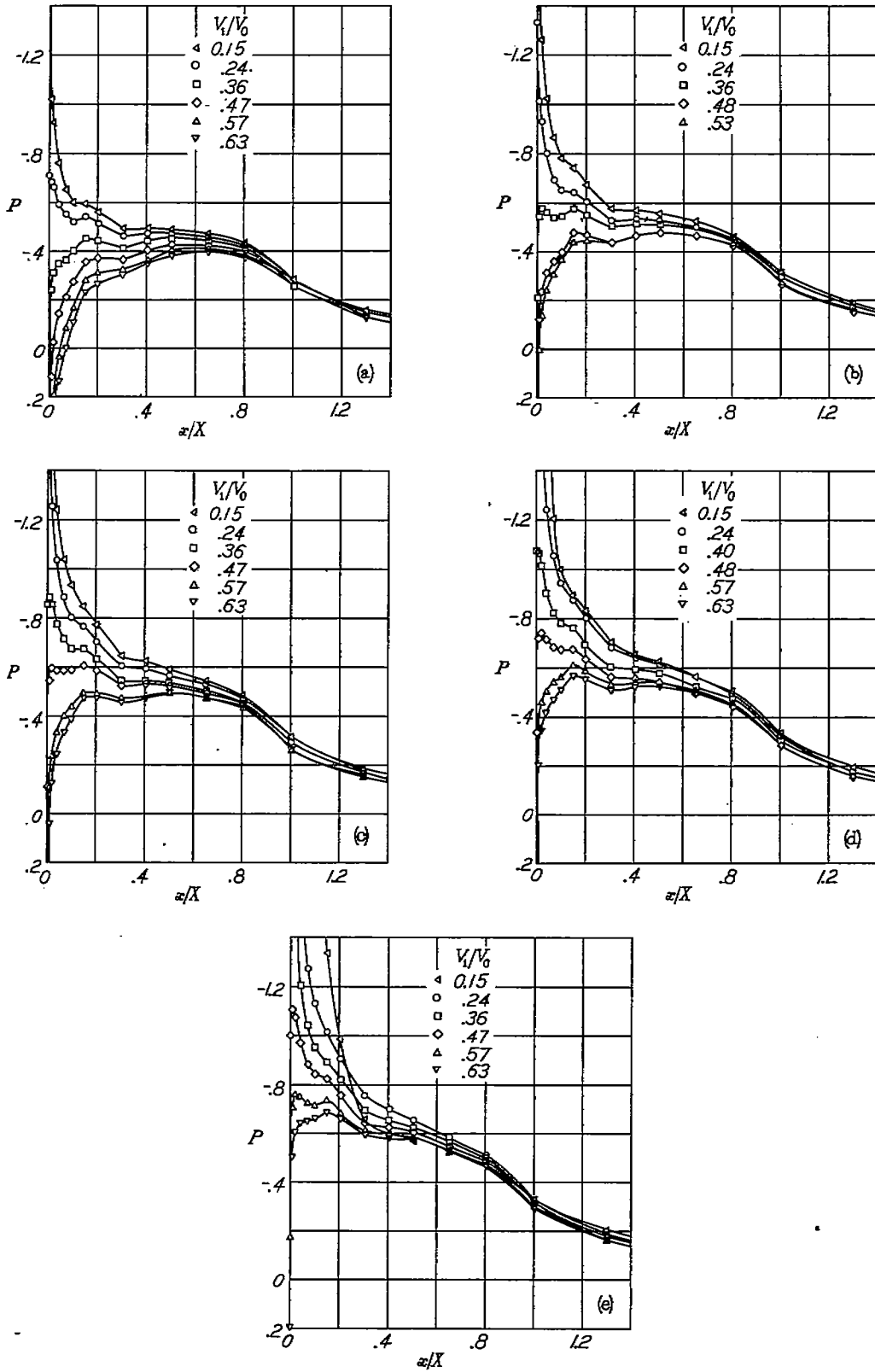
FIGURE 25.—Pressure distributions over the NACA 1-70-050 nose inlet. M_0 = 0.30 .
