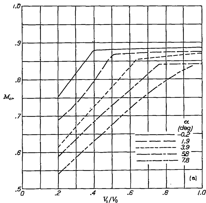
(a) NACA 1-40-200 nose inlet.
