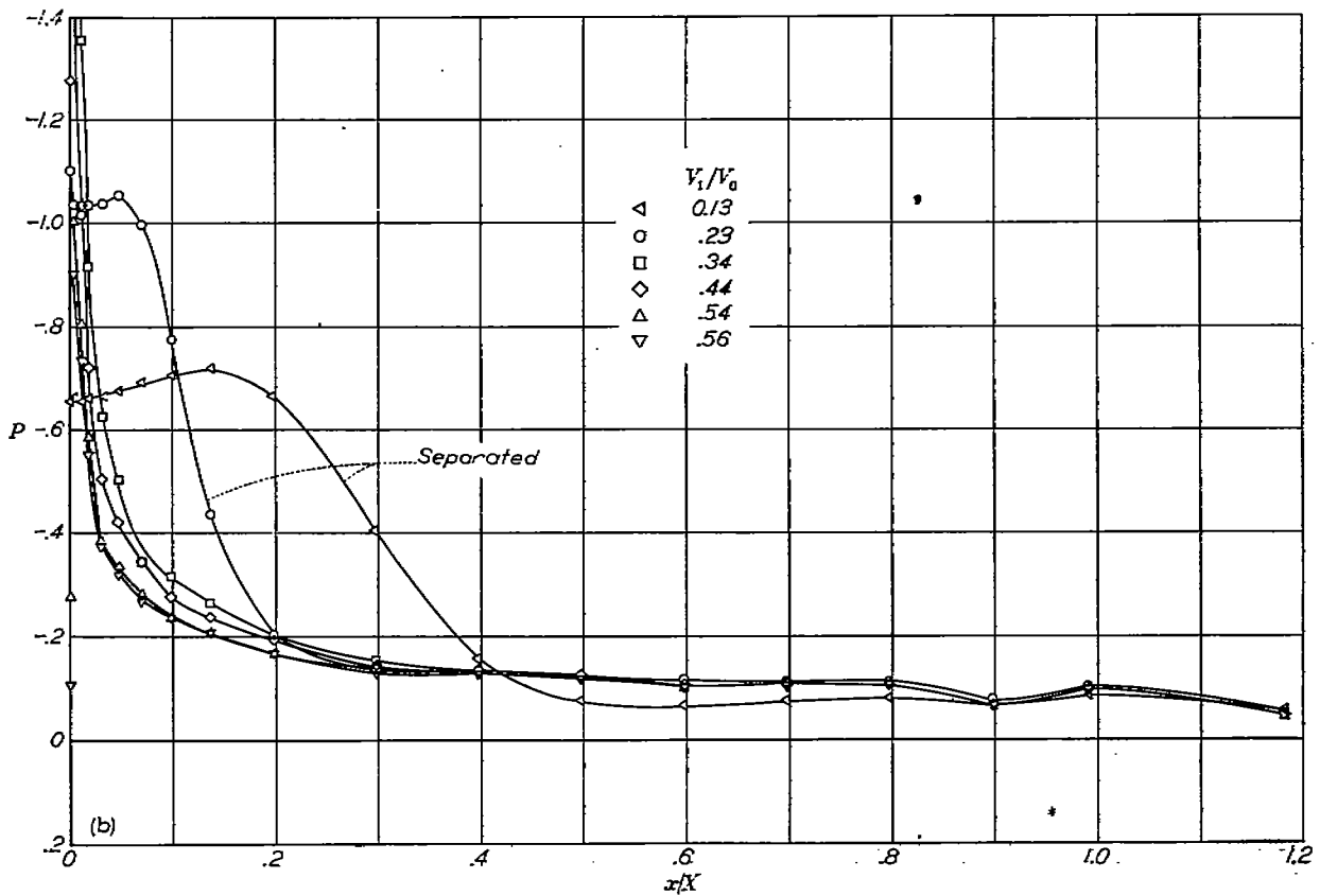
FIGURE 23.—Pressure distributions over the NACA 1-70-150 nose inlet.
