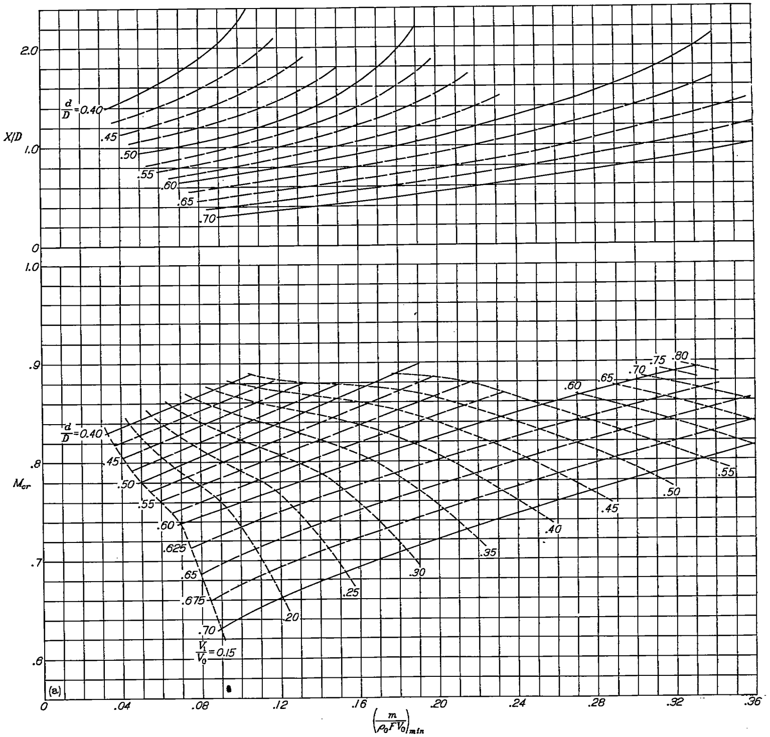
FIGURE 31.—Selection charts for NACA 1-series nose inlets.
