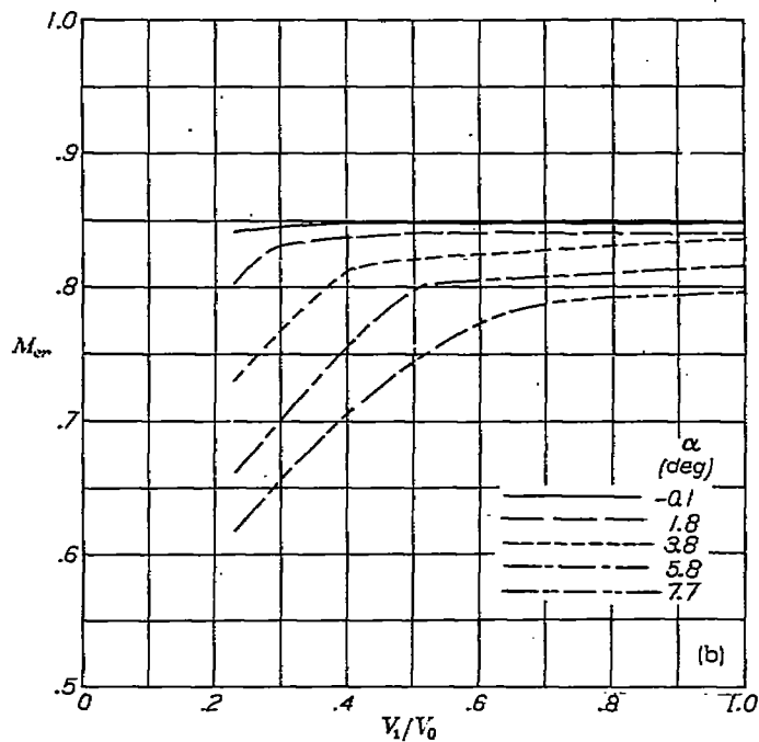
(b) NACA 1-40-180 nose inlet.
