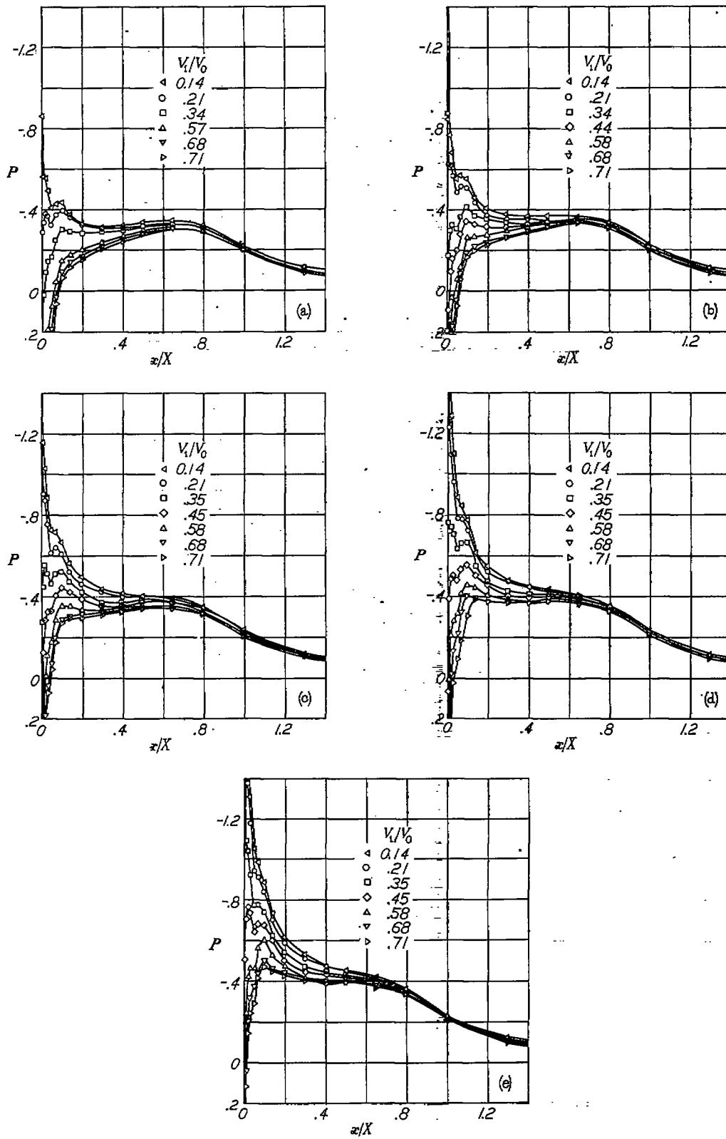
FIGURE 20.—Pressure distributions over the NACA 1-60-075 nose inlet. M_1 = 0.40 .
