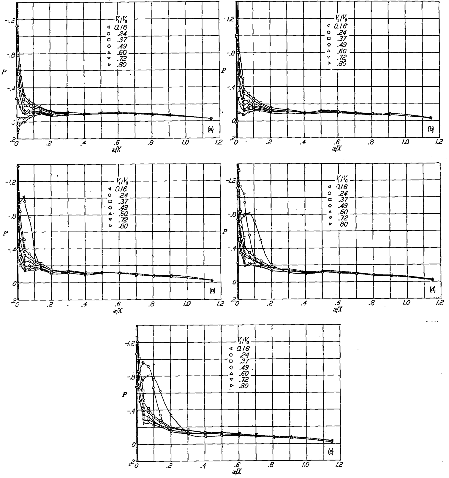
(a) \alpha = -0.1^\circ . (b) \alpha = 1.9^\circ . (c) \alpha = 3.9^\circ . (d) \alpha = 5.9^\circ . (e) \alpha = 7.9^\circ . FIGURE 17.—Pressure distributions over the NACA 1-60-200 nose inlet. M_0 = 0.30 .
