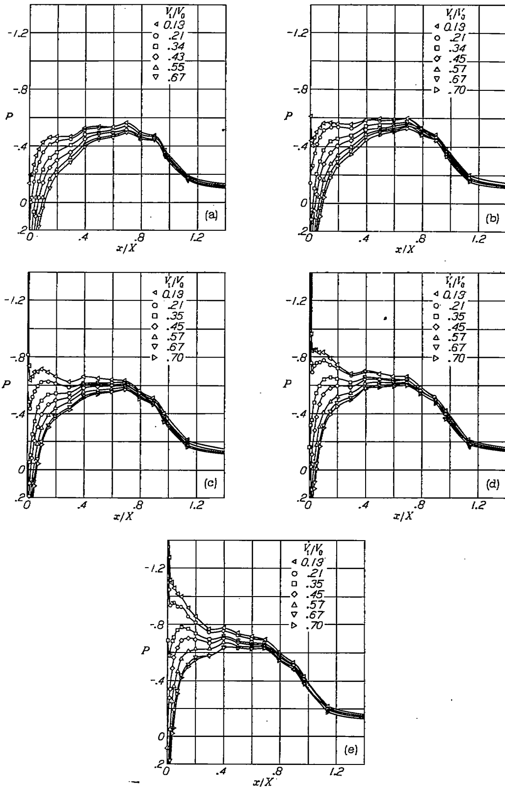
(a) \alpha = -0.2^\circ . (b) \alpha = 1.8^\circ . (c) \alpha = 3.8^\circ . (d) \alpha = 5.8^\circ . (e) \alpha = 7.8^\circ . FIGURE 21.—Pressure distributions over the NACA 1-60-050 nose inlet. Ma = 0.40 .
