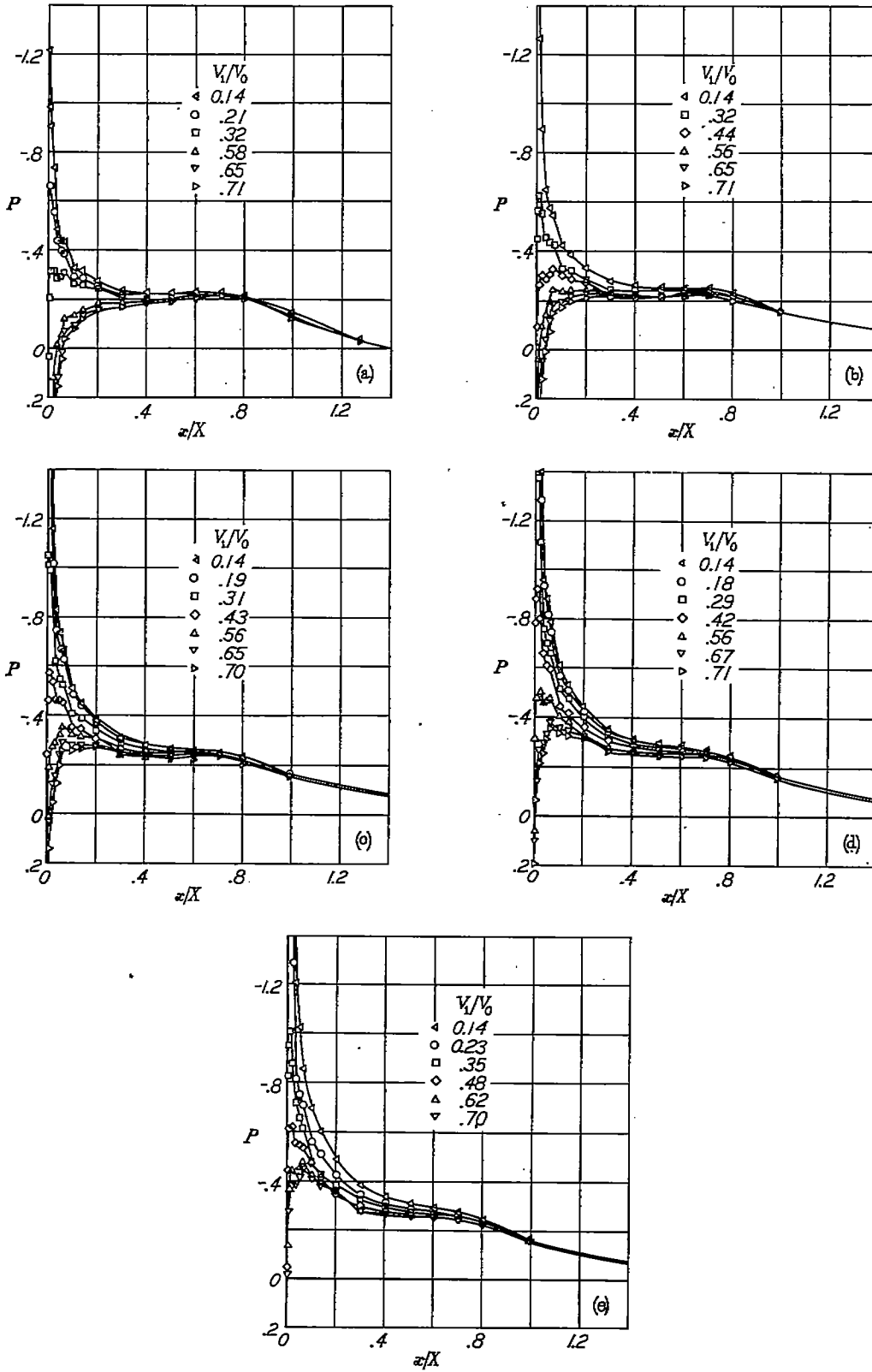
(a) \alpha = -0.2^\circ . (b) \alpha = 1.9^\circ . (c) \alpha = 3.9^\circ . (d) \alpha = 5.8^\circ . (e) \alpha = 7.8^\circ . FIGURE 19.—Pressure distributions over the NACA 1-80-100 nose inlet. M_0 = 0.40 .
