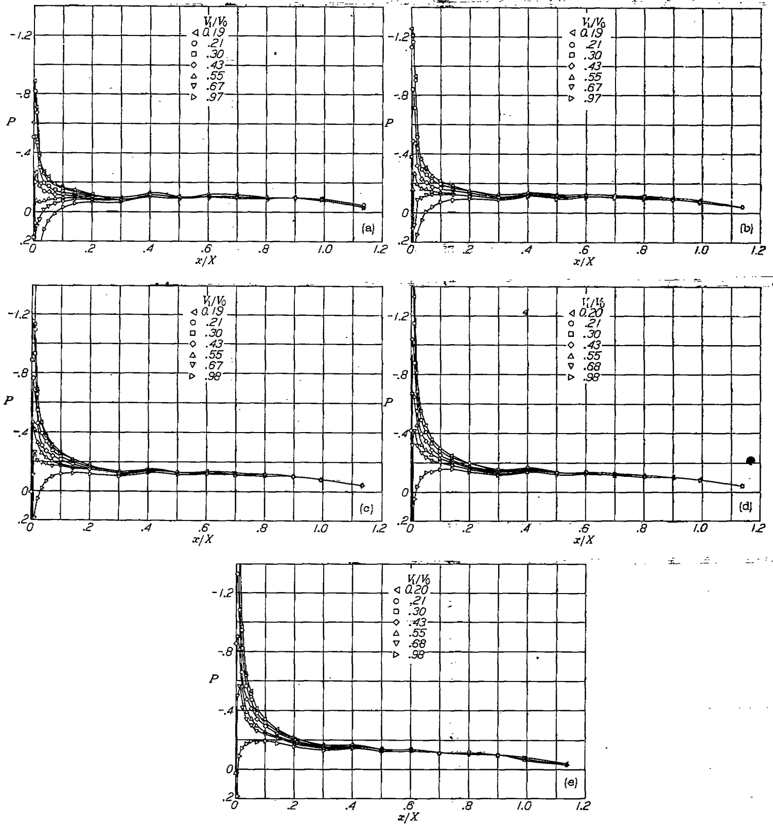
(a) \alpha = -0.1^\circ . (b) \alpha = 1.8^\circ . (c) \alpha = 3.9^\circ . (d) \alpha = 5.8^\circ . (e) \alpha = 7.9^\circ . FIGURE 12.—Pressure distributions over the NACA 1-50-200 nose inlet. M_0 = 0.40 .
