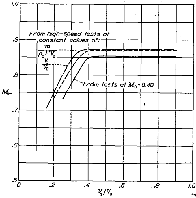
FIGURE 44.—Critical Mach numbers obtained from tests at M_0=0.40 (fig. 18(b)) and from tests at high speed (fig. 42) for the NACA 1-50-150 nose inlet. \alpha=0.2^\circ .
