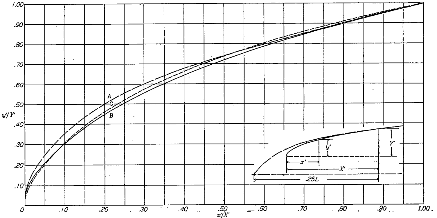
FIGURE 1.—Comparison of nondimensional profiles and proportions of the three high-critical-speed nose inlets developed in tests of reference 2.
