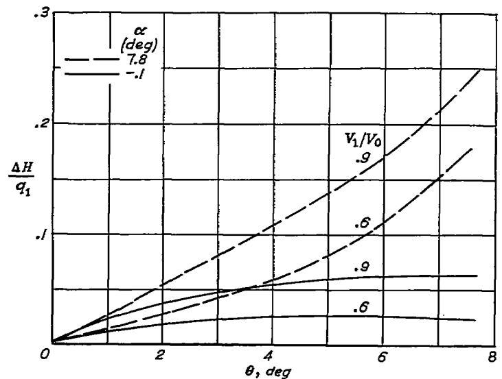
FIGURE 50.—Variation of internal total-pressure loss with diffuser angle. X/D=1.6 ; M_0=0.40 .
