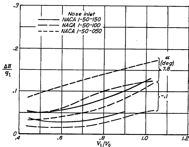
FIGURE 52.—Variation of internal total-pressure loss with inlet-velocity ratio for nose inlets of \frac{d}{D} = 0.5 . M_0 = 0.40 ; \theta = 3.8^\circ .
