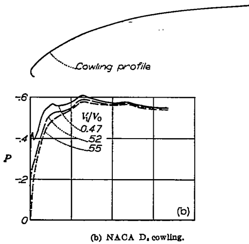
FIGURE 38.—Pressure distributions over NACA D 1 and D 2 cowlings. (Data from references 5 and 6.) \alpha=0^\circ .
