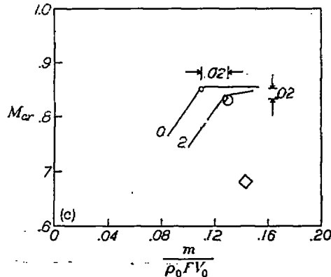
FIGURE 33.—Comparison of three NACA 1-series nose inlets selected for one application. (See example in text.) Curves are estimated.
