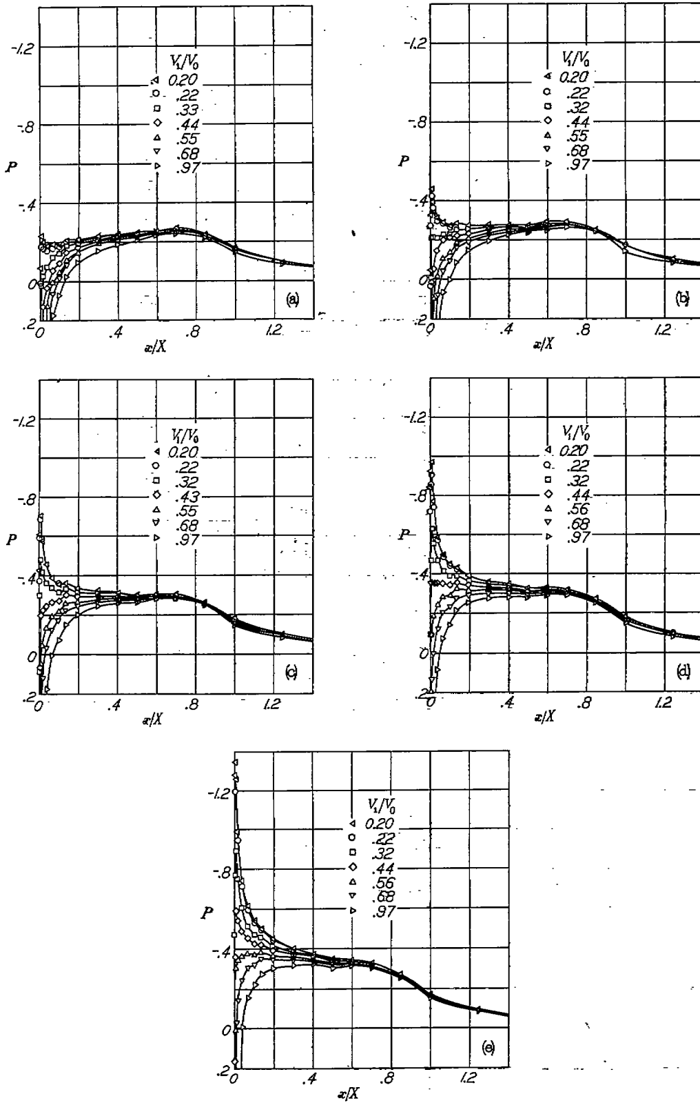
(a) \alpha = -0.2^\circ . (b) \alpha = 1.8^\circ . (c) \alpha = 3.9^\circ . (d) \alpha = 5.8^\circ . (e) \alpha = 7.8^\circ . FIGURE 14.—Pressure distributions over the NACA 1-50-100 nose inlet. M_0 = 0.40 .
