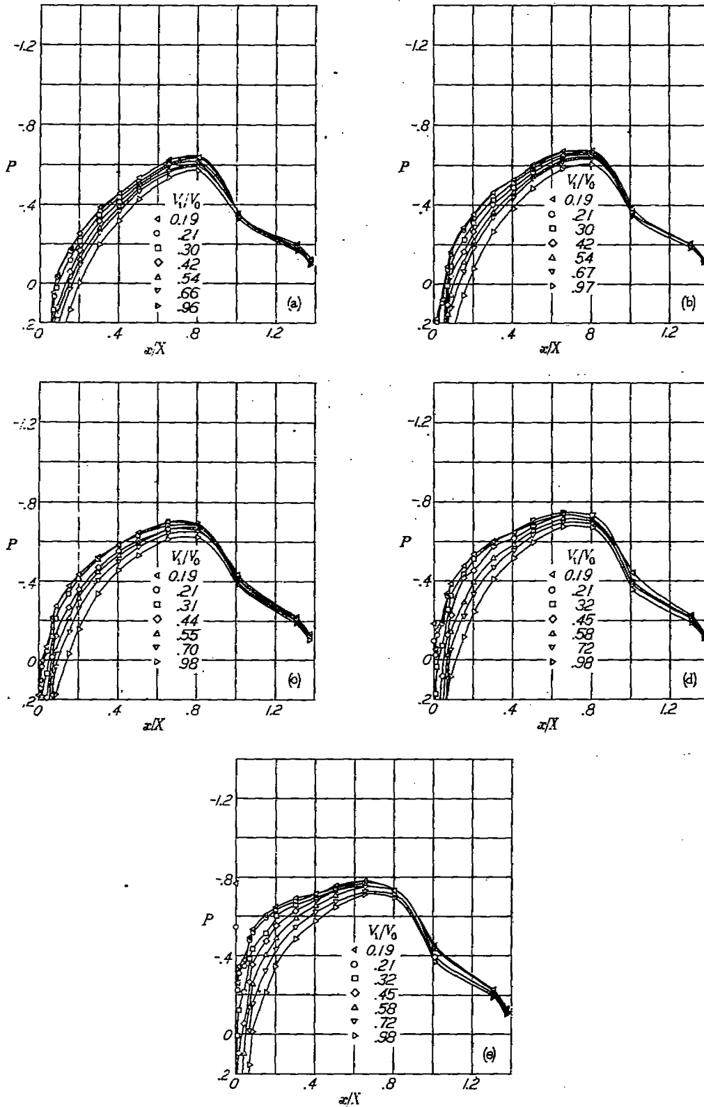
FIGURE 15.—Pressure distributions over the NACA 1-60-030 nose inlet. M_1 = 0.40 .
