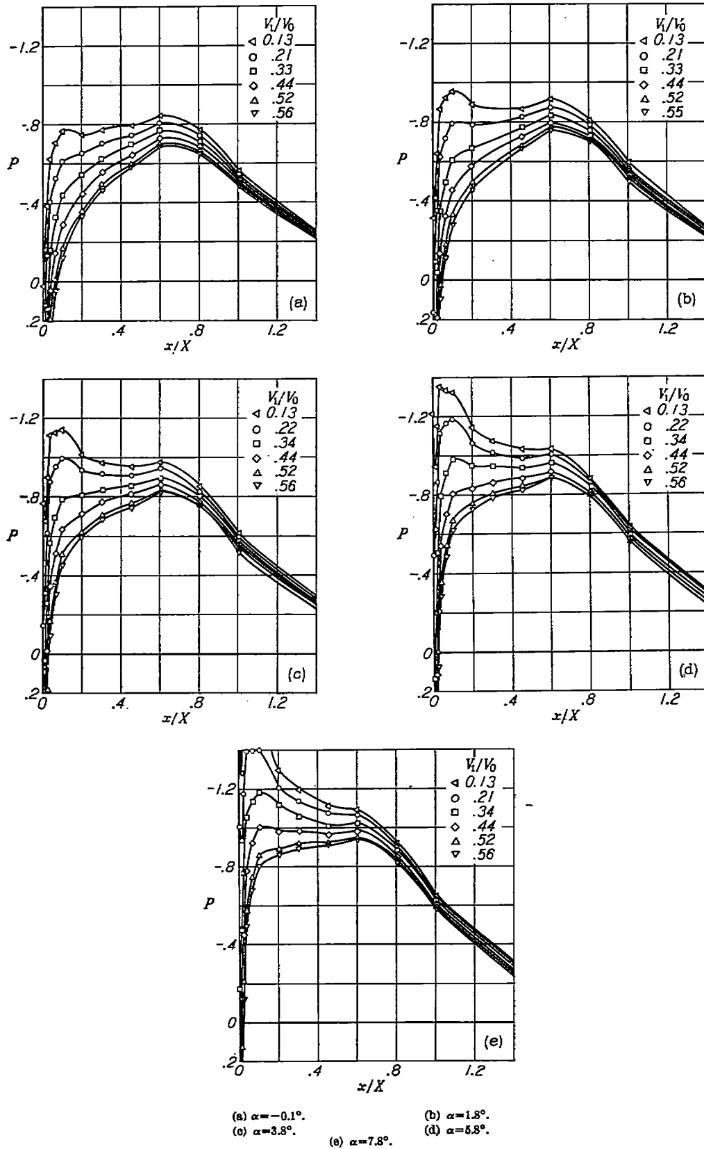
FIGURE 55.—Pressure distributions over the NACA C cowling with increased lip radius. M_1=0.40 .
