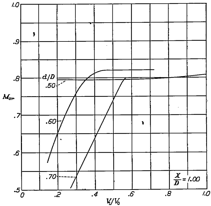
FIGURE 29.—Critical Mach number characteristics of NACA 1-series nose inlets tested, grouped according to length ratio. \alpha = 0^\circ .
