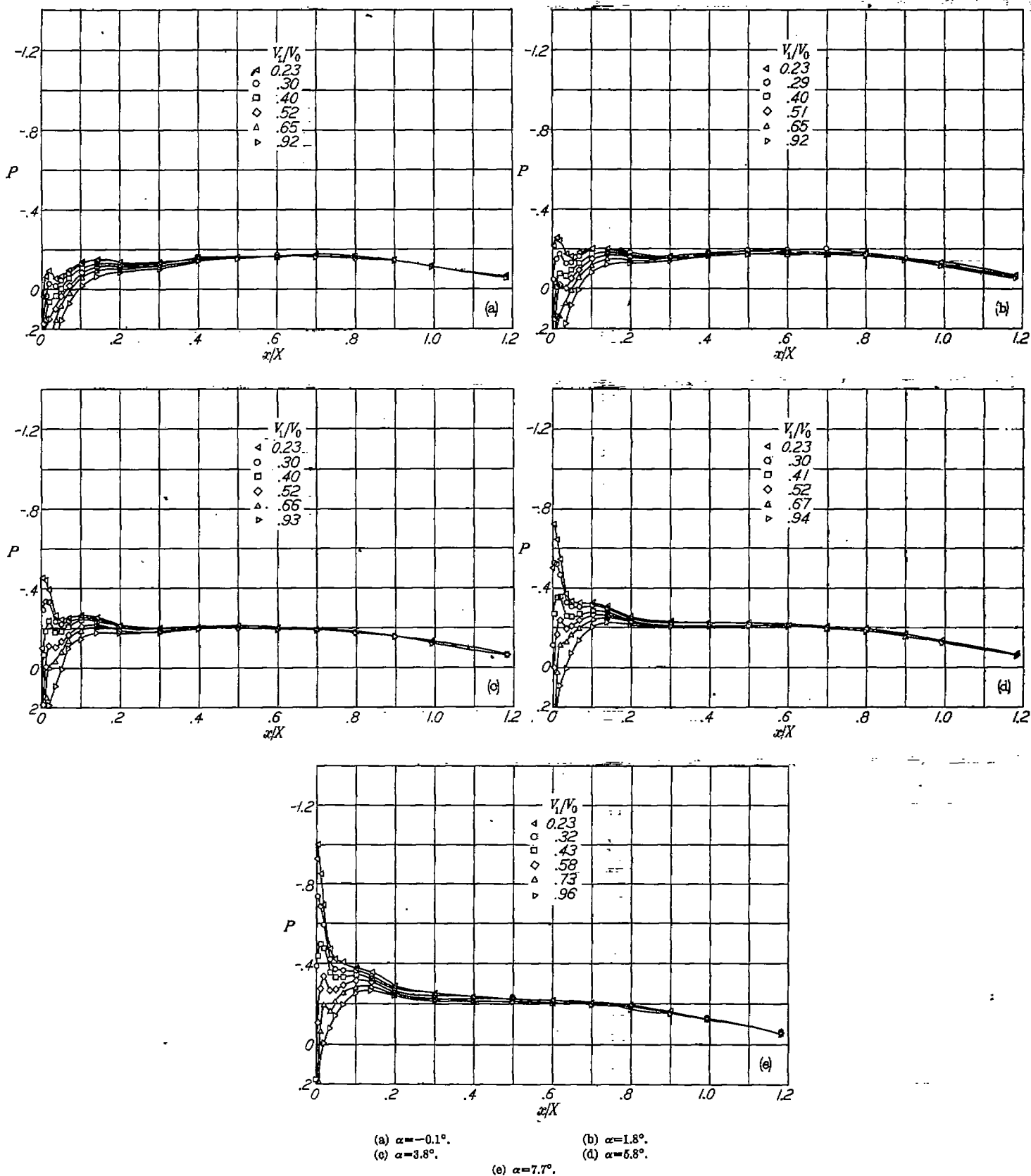
FIGURE 10.—Pressure distributions over the NACA 1-40-150 nose inlet. M_0=0.4
