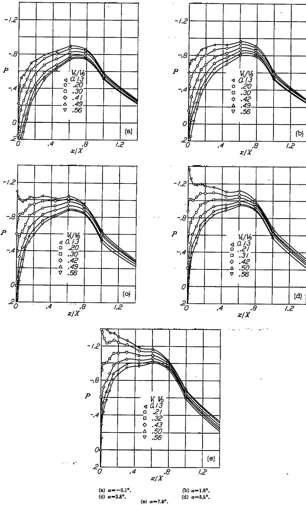
FIGURE 54.—Pressure distributions over the NACA 1-70-030 nose inlet with increased lip radius. M_1=0.40 .
