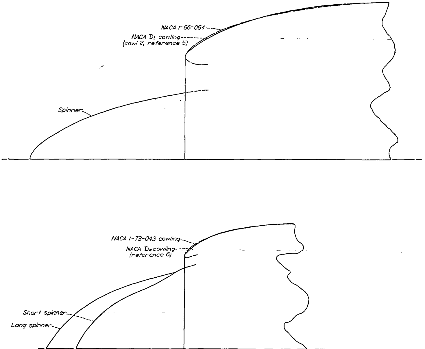
FIGURE 37.—NACA cowlings developed for use with large spinners. NACA 1-series cowlings of similar proportions superimposed for comparison of profiles.
