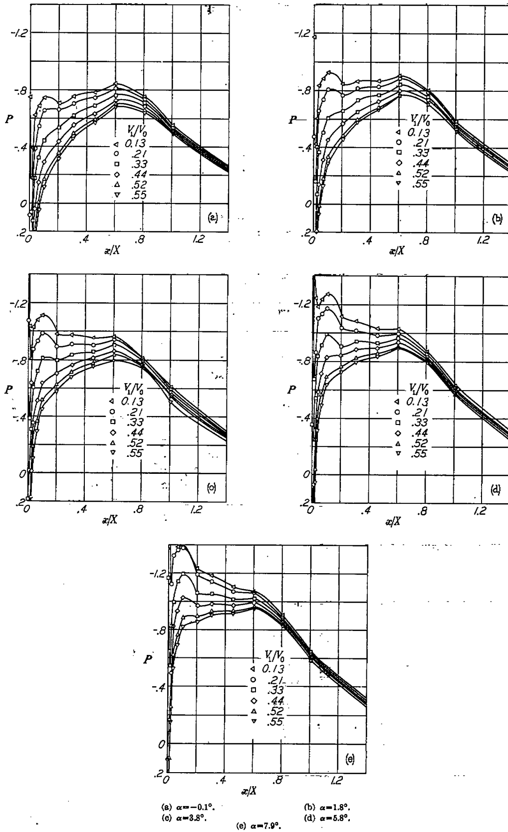
FIGURE 34.—Pressure distributions over the NACA C cowl. M_0=0.40 .
