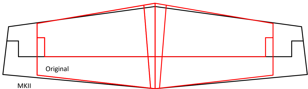
Figure 2, Horizontal Stabilizer Comparison
