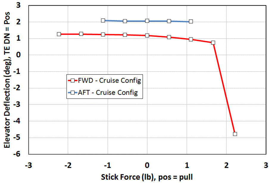
Figure 14, Original Stabilizer, Elevator Deflection with Stick Force
