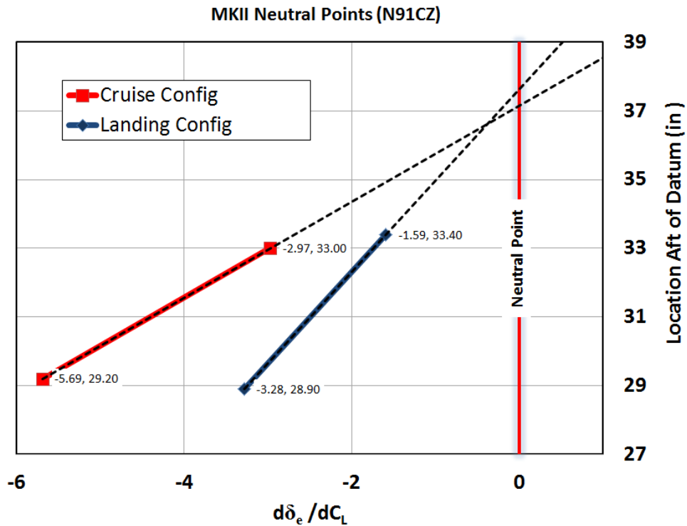
Figure 3, MKII Stabilizer Neutral Point
