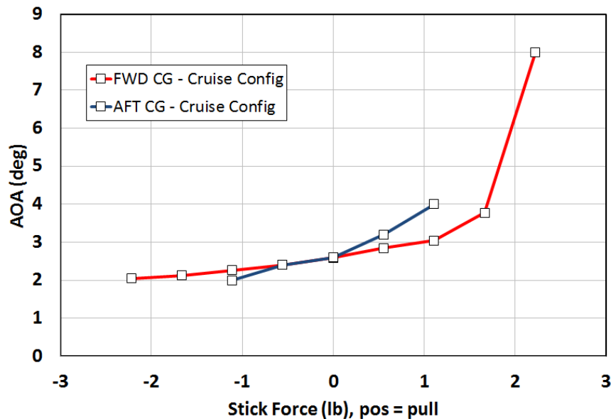
Figure 16, Original Stabilizer, Angle of Attack Sensitivity to Stick Force
