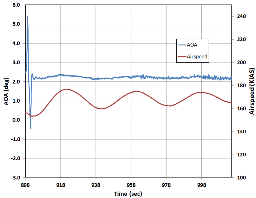
Figure 9, Original Stabilizer, Phugoid triggered by Doublet
