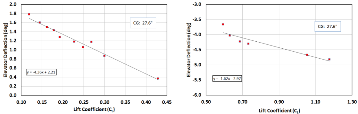
Figure 17, Original Stabilizer Neutral Point Testing in Cruise Configuration
