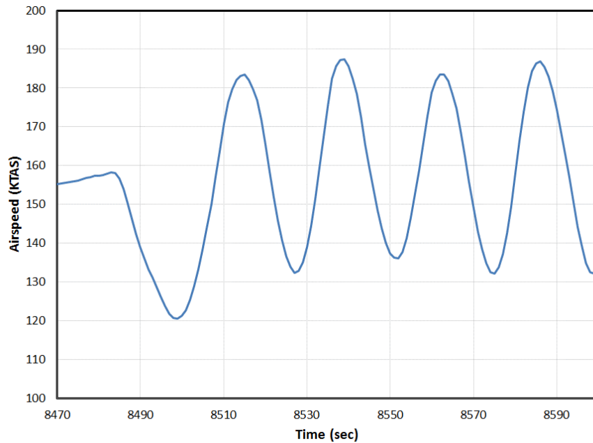
Figure 12, Original Stabilizer, Phugoid, Cruise, AFT CG
