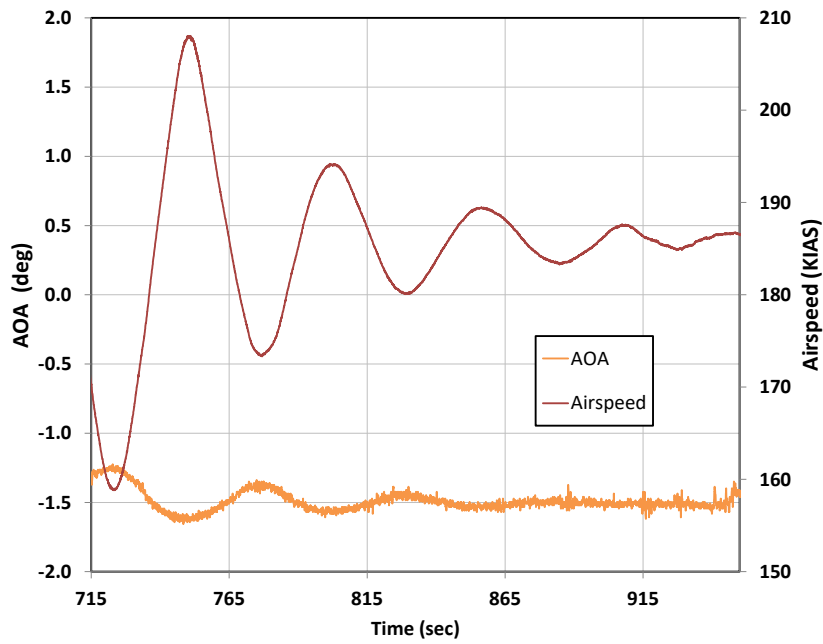
Figure 10, MKII Stabilizer, Phugoid, Cruise, FWD CG
