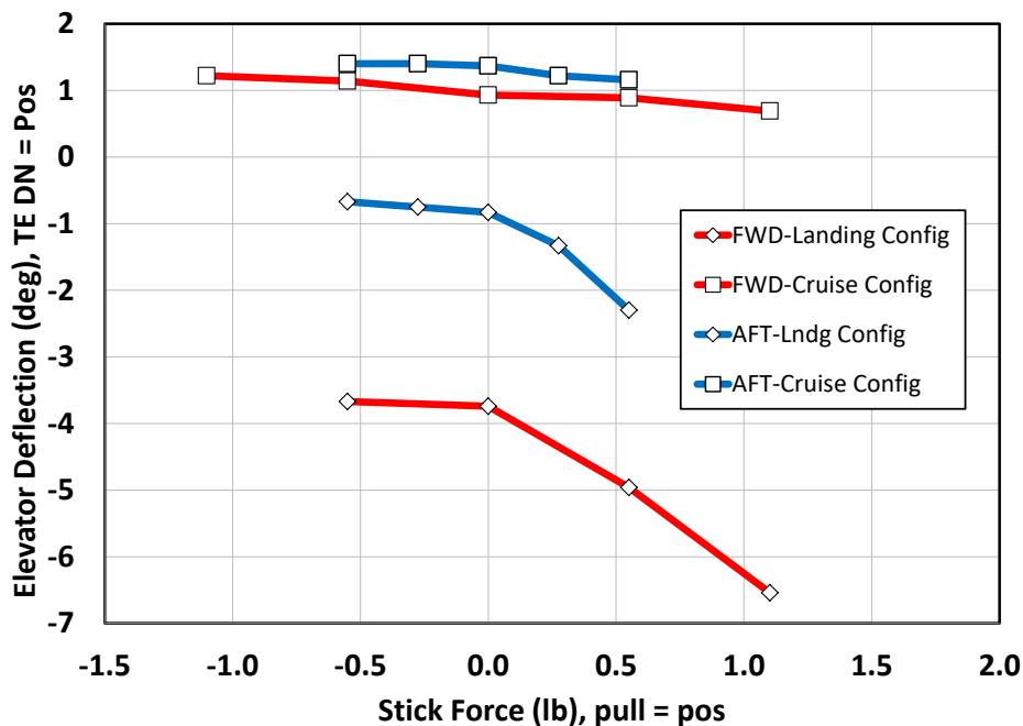
Figure 13, MKII Stabilizer Elevator Deflection with Stick Force
