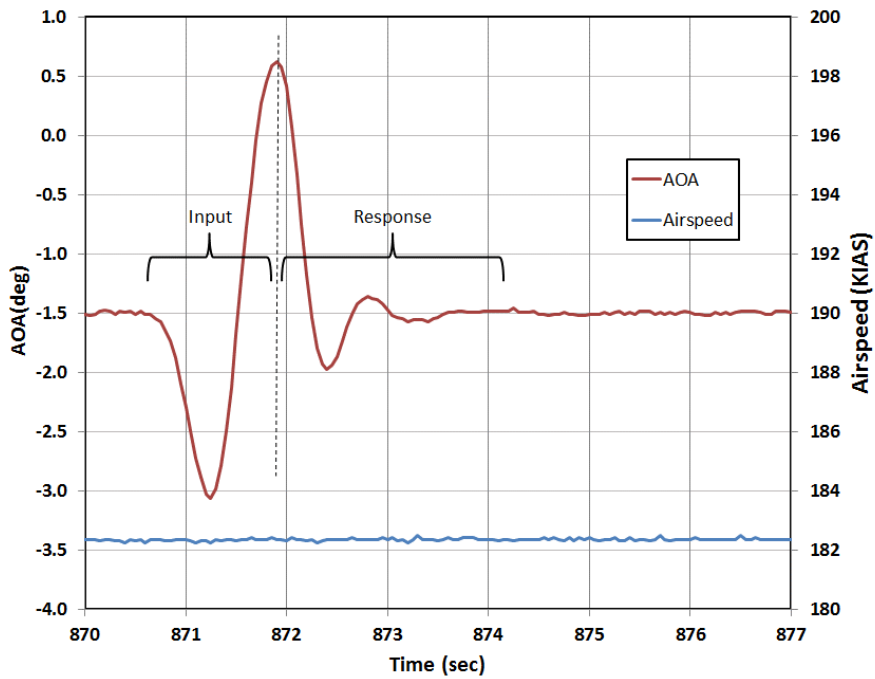
Figure 7, MKII Stabilizer, Short Period, Cruise, FWD CG
