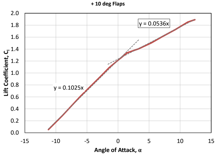
Figure 4, NLF(1)-0215F Section Lift Coefficient, Flaps +10 (Somers, 1981)
