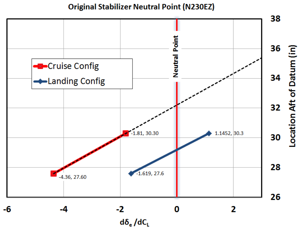
Figure 6, Original Stabilizer Neutral Point
