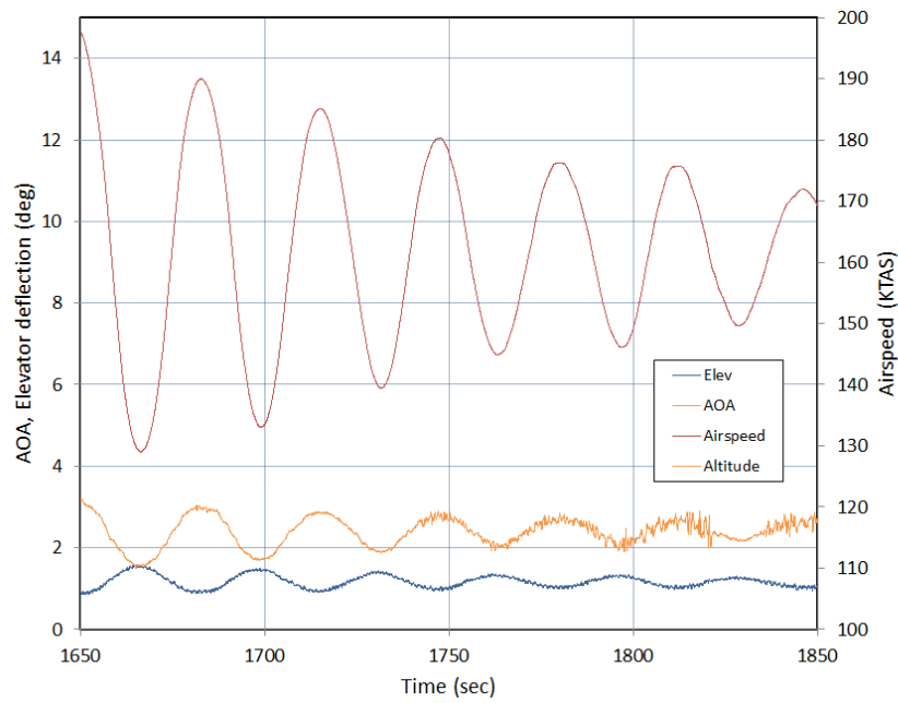
Figure 11, Original Stabilizer, Phugoid, Cruise, FWD CG
