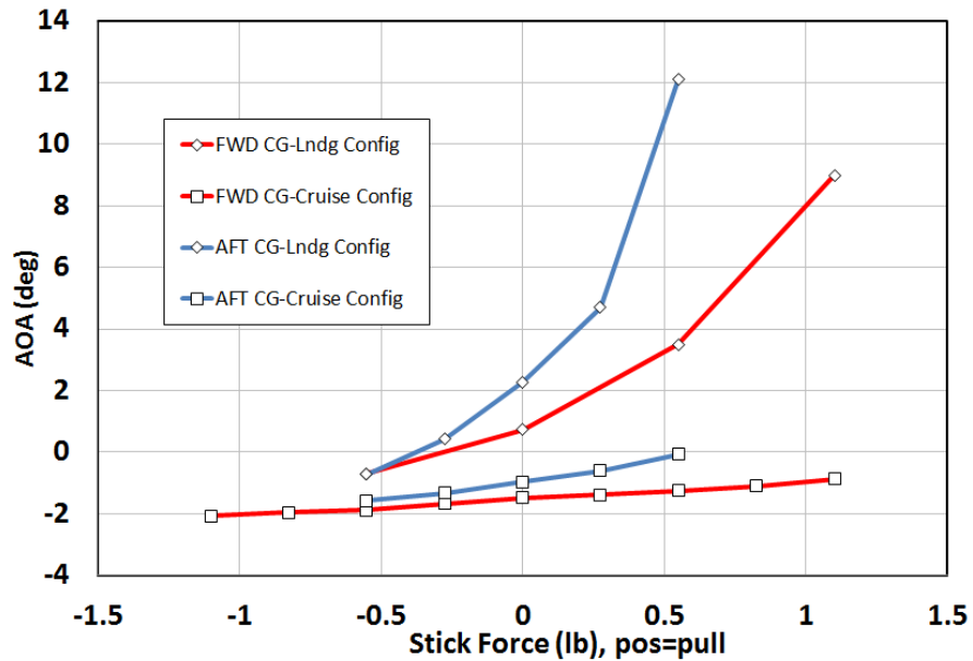
Figure 15, MKII Stabilizer, Angle of Attack Sensitivity to Stick Force
