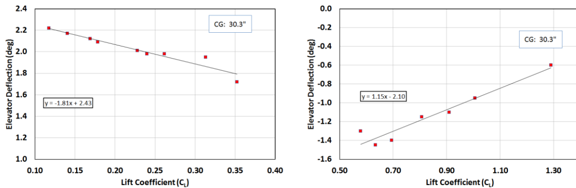
Figure 18, Original Stabilizer Neutral Point Testing in Landing Configuration
