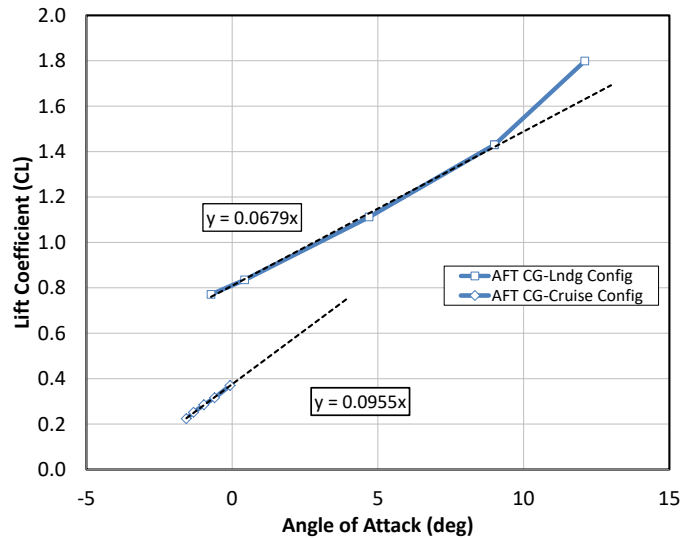
Figure 5, Lift Curve Slopes, Cruise, Landing Configurations
