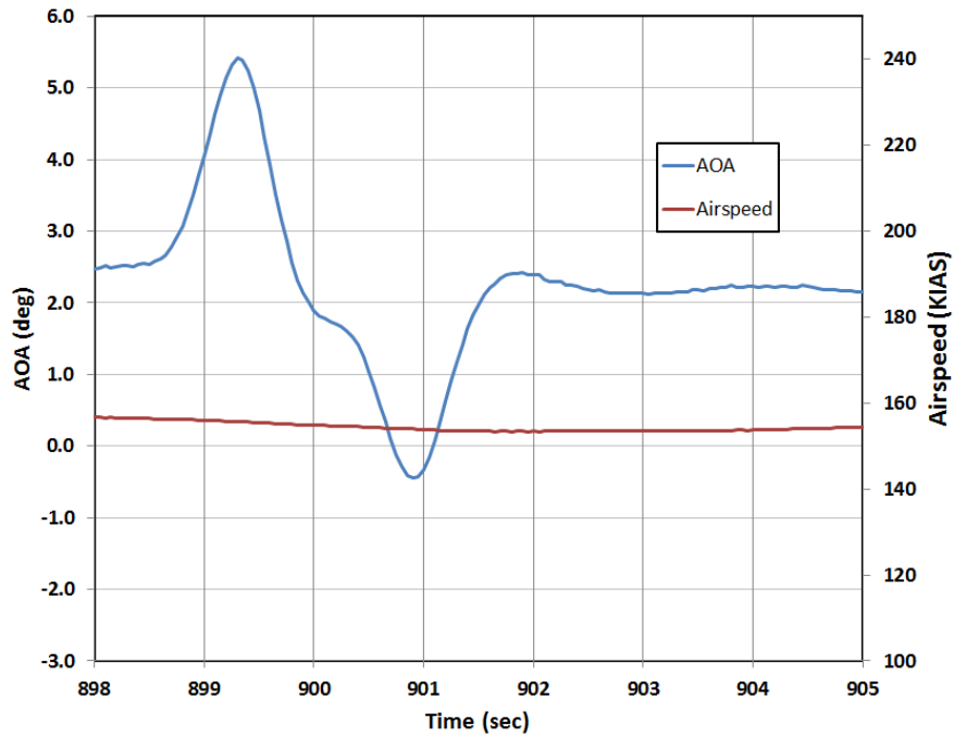
Figure 8, Original Stabilizer, Short Period, Cruise, FWD CG
